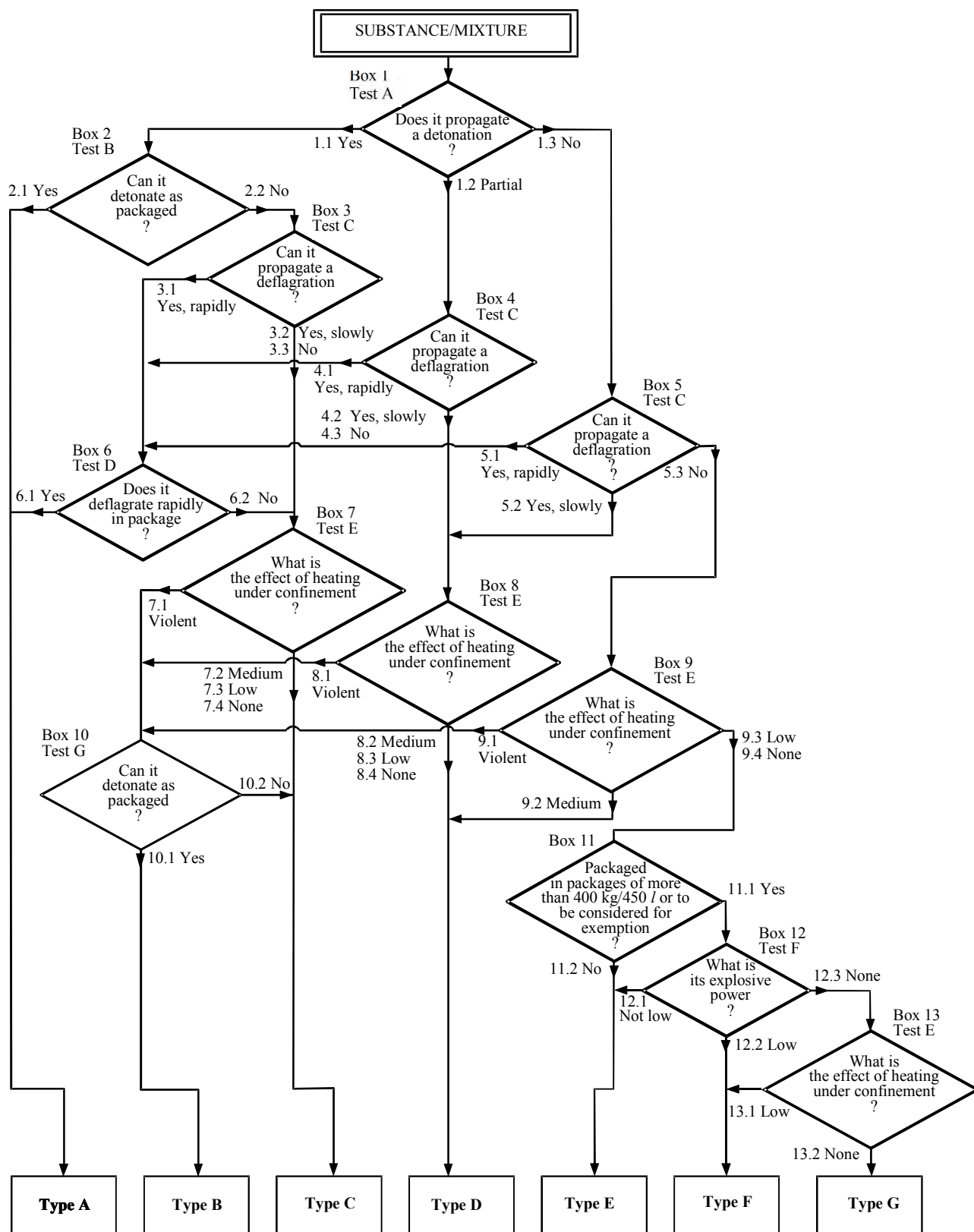
Figure VIII.13.1. Decision logic for classifying organic peroxides.
