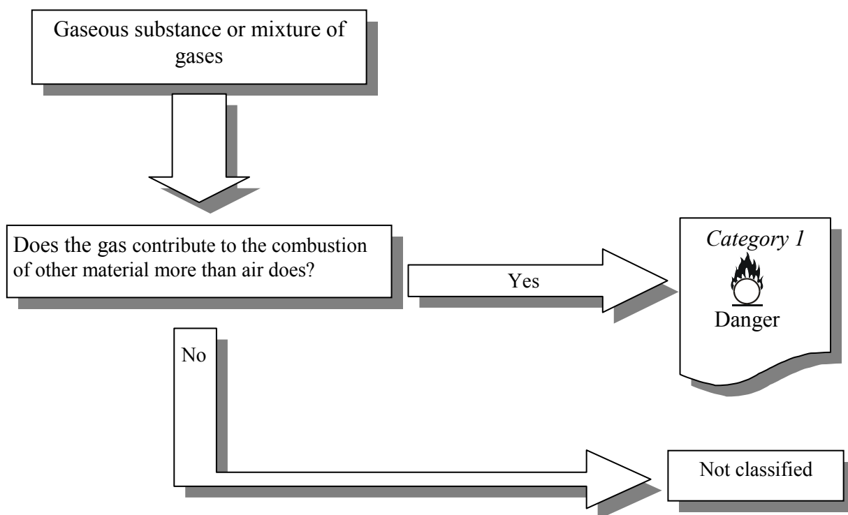
Figure VIII.4.1. Decision logic for classifying oxidizing gases.
