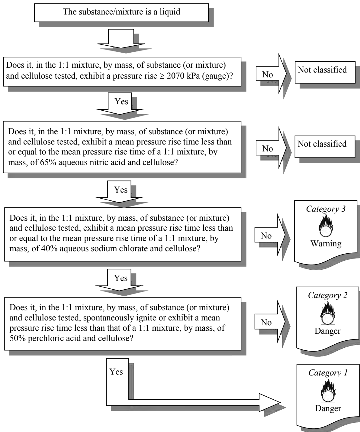
Figure VIII.12.1. Decision logic for classifying oxidizing liquids.
