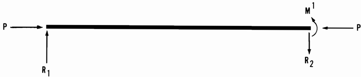
Figure A2-2. Beam Buckling Example
