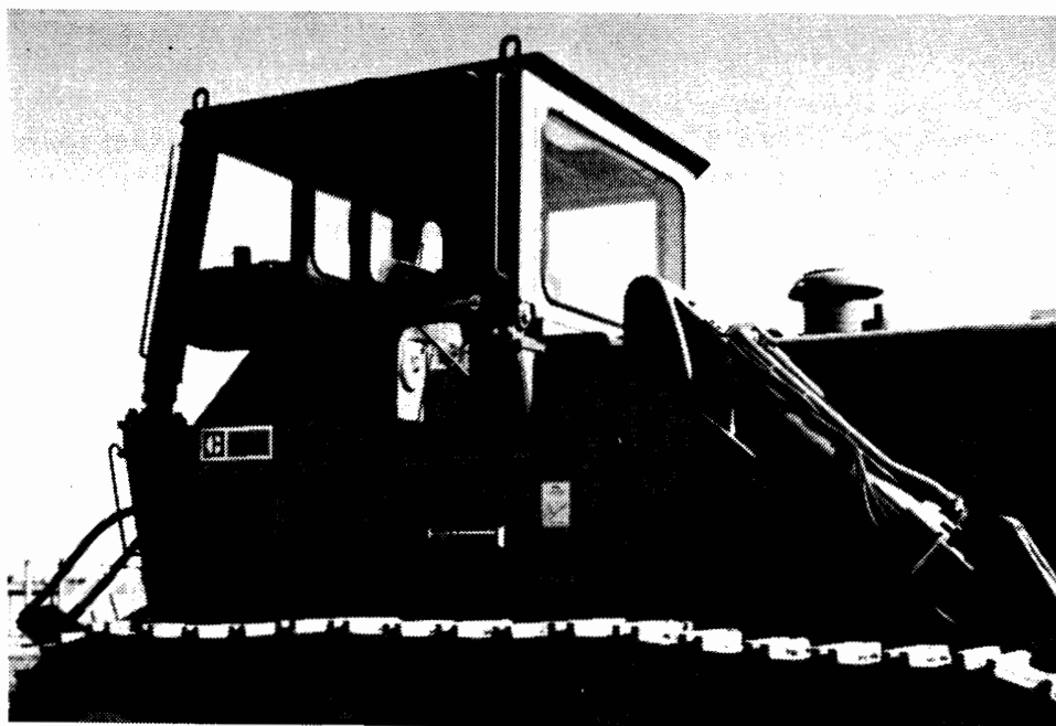
Figure 4-26. Saf-T-Cab ROPS Cabs on Caterpillar Motor Grader and on Caterpillar Crawler Loader
