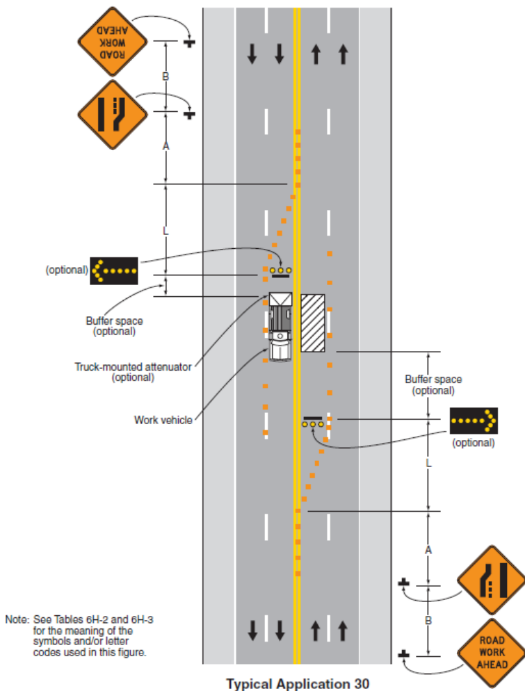
Figure 6H-30. Interior Lane Closure on a Multi-Lane Street (TA-30)
