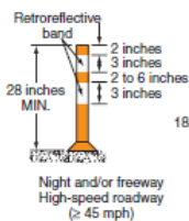
Figure 6F-7. Channelizing Devices
